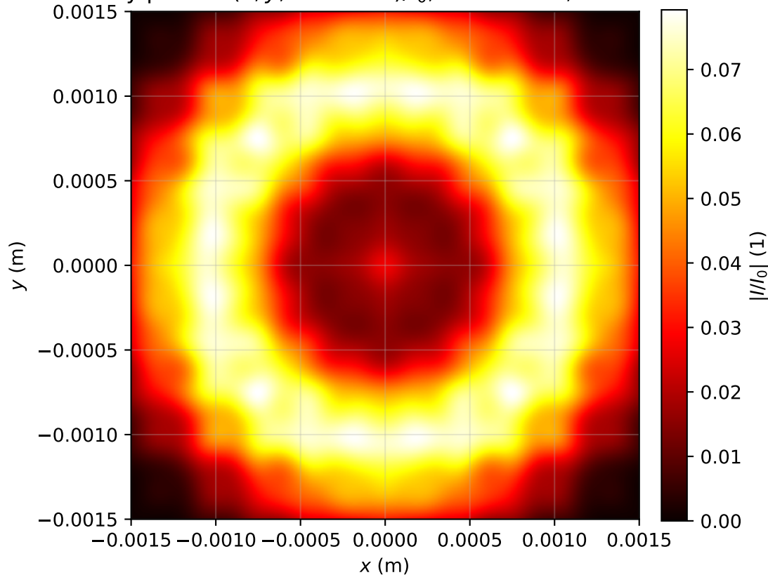
Intensity profile I(x, y, z = 3.105)/I_0 , P_{in}=6.5P_{cr} , artificial time
